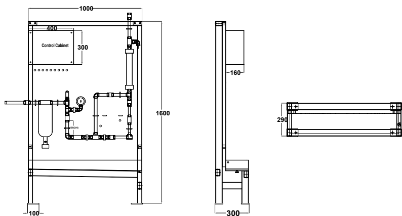
WATER FLOW CONTROLLER
